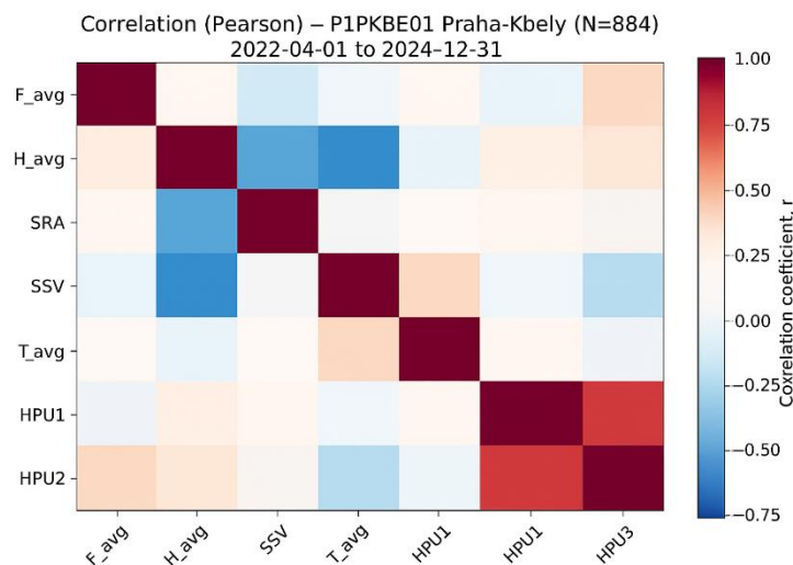
Fig 3 Pearson correlation matrix of all measured variables at the P1PKBE01 Praha-Kbely station ( N = 884 ) for the period 1 April 2022–31 December 2024
