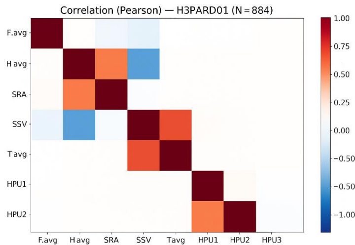
Fig 5 Pearson correlation matrix of all measured variables at the station H3PARD01 Pardubice ( N = 884 ) for the period 1 April 2022–31 December 2024.
