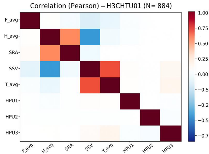
Fig 4 Pearson correlation matrix of all measured variables at the H3CHTU01 Chotusice station ( N = 884 ) for the period 1 April 2022–31 December 2024.
